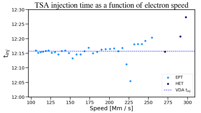
Fig. C.2. A scatter plot showing the injection times acquired by a simple time-shift ( t_{inj} = t_{onset} - L/v ) for EPT and HET onset times. The horizontal dashed blue line represents the injection time predicted by VDA (Fig. C.1). Largely static injection time as a function of energy, assuming the electrons travelled the same path, suggests a common time of injection.
