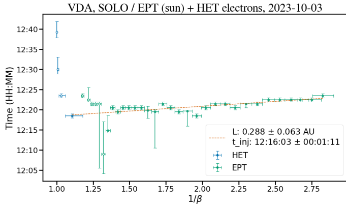
Fig. C.1. Velocity dispersion analysis plot on SoLO EPT+HET electron onset times. Horizontal axis corresponds to the inverse unitless velocity of the electrons ( 1/\beta = c/v ) and the vertical axis shows time. Data points mark the onset times, with horizontal error bars displaying the width of each energy channel and vertical error displaying the uncertainty related to the onset times. The dashed orange line shows a linear fit applied on the selected (solid circles) onset times using orthogonal distance regression (ODR) algorithm. Onset times marked with hollow circles are not considered to the fit for their deviance from the general velocity dispersion trend.
