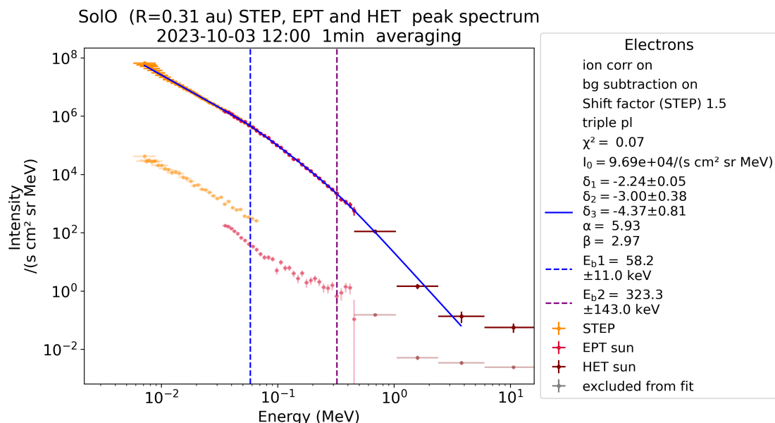
Fig. 7. Energetic electron peak intensity spectrum measured by SoLo/EPD. The lower and fainter points represent the pre-event background, while the higher points represent the peak intensity measured by STEP, EPT and HET. The spectrum is fit with a triple power-law, excluding the last energy channel of HET.
