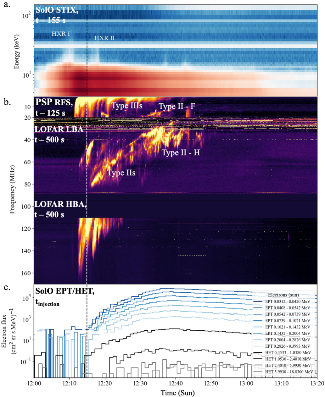
Fig. 2. X-ray spectrogram, composite dynamic spectrum of a complex radio event and energetic electron time series observed on 3 October 2023. (a) X-ray spectrogram from SolO/STIX showing the onset of the flare and the presence of two hard X-ray peaks: HXR I and HXR II. (b) The dynamic spectrum consists of spectra from PSP/RFS (1–20 MHz), LOFAR LBA (10–90 MHz) and LOFAR HBA (110–170 MHz). The labels 'F' and 'H' refer to fundamental and harmonic emissions, respectively. (c) Time-series of energetic electrons measured by SolO EPT & HET from the sunward direction (where the first-arriving electrons are observed) and at multiple energy channels. The time represents the injection time for each channel. The spectra are time-shifted to correspond to time at the Sun so that they can be compared directly to the electron injection times.
