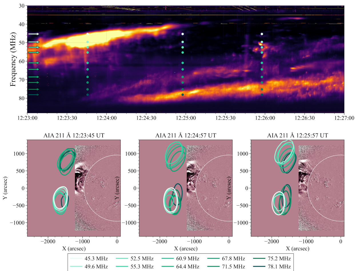
Fig. 3. The type II burst in dynamic spectrum and radio images. The top panel shows a zoomed in dynamic spectrum of the onset of the type II harmonic lanes. The arrows located to the left of this panel represent the frequency subbands that were imaged in the bottom panels. The bottom panels show the 70% radio contours at the time and frequencies denoted in the top panel using the same colouring, overlaid on AIA 211 Å running difference images of the eruption. The radio contours and AIA images have the same time stamps, as shown in the panels. The time labels in this figure are UT observer times.
