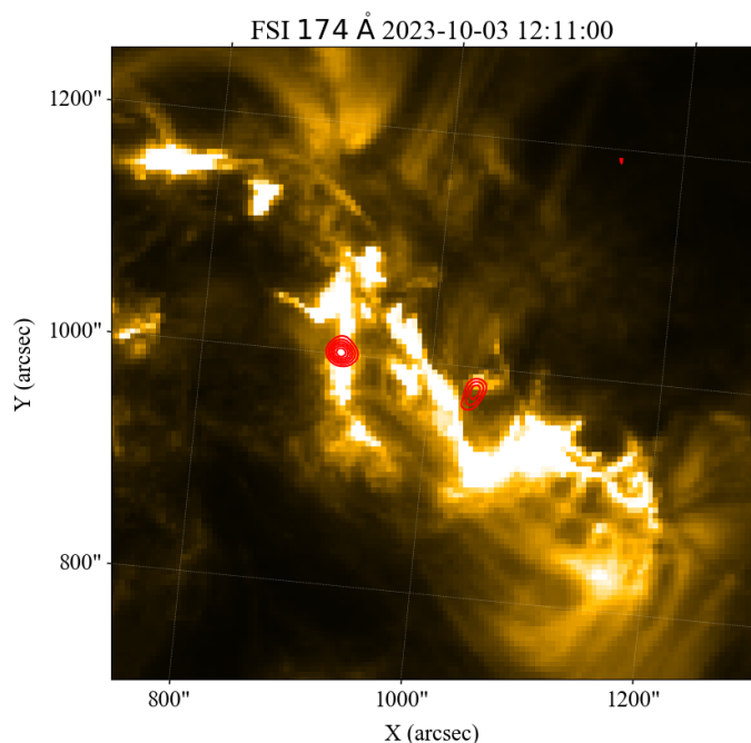
Fig. A.1. EUV image of the Sun as viewed from SolO. Overlaid on the EUV image are the STIX HXR contours in red from 40-90% of the maximum intensity level at energies of 20–40 keV and integrated time period of 12:17:30-12:20:30 UT.
